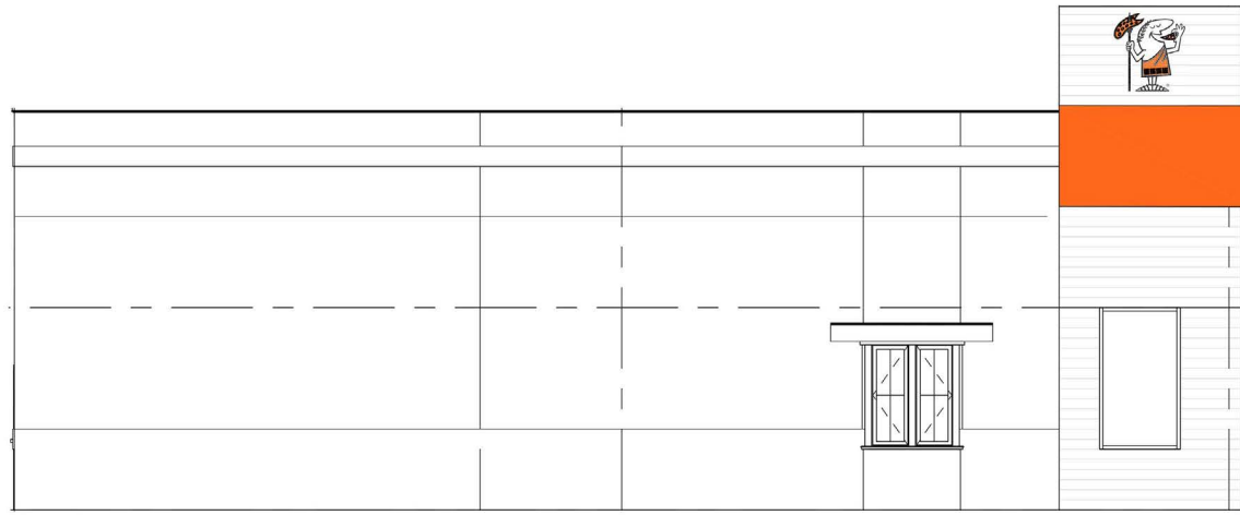
△ SIDE SIGNAGE ELEVATION SCALE: 1/4"=1'-0"
