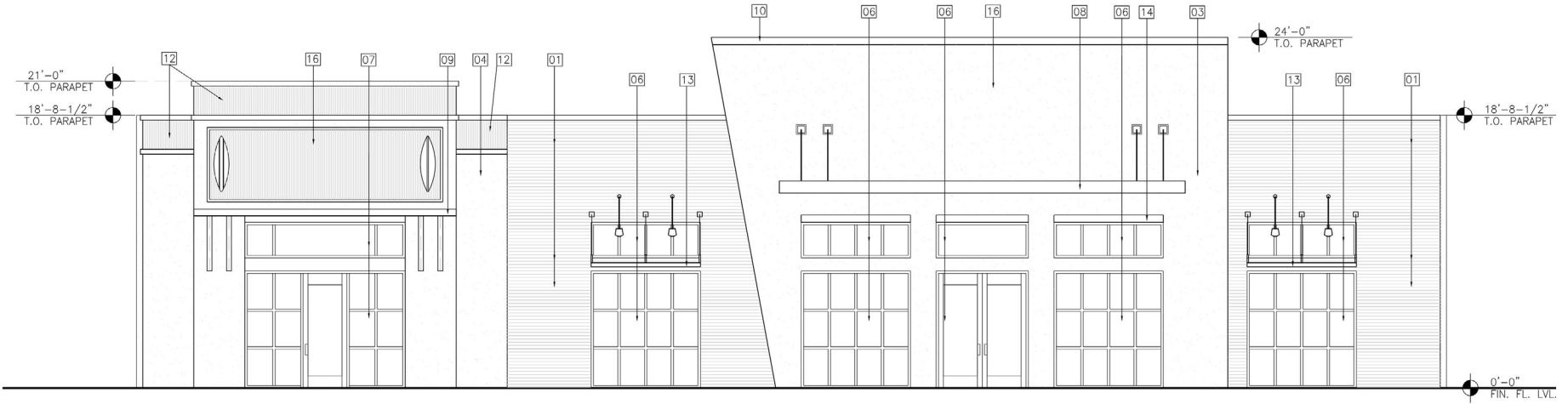
1 PROPOSED WEST ELEVATION CHANGES A2.0 SCALE: 1/4"=1'-0"
