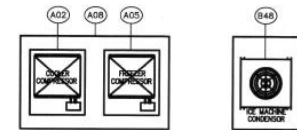
EQUIPMENT LAYOUT PLAN SCALE: 1/4" = 1'-0"
