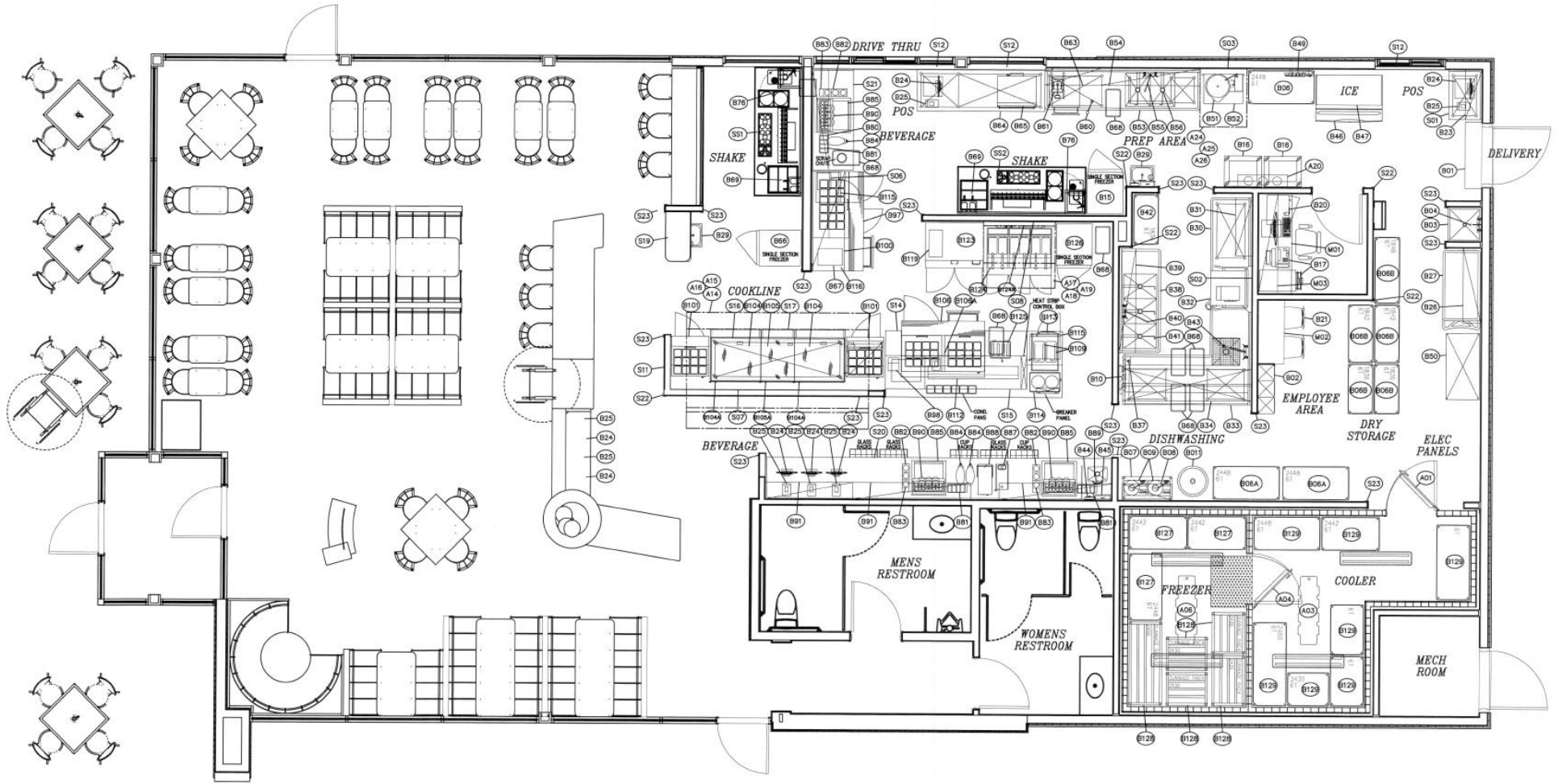
EQUIPMENT LAYOUT PLAN SCALE: 1/4" = 1'-0"
